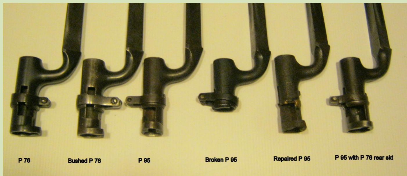
A comparison of Martini sockets
