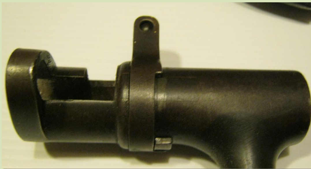
The filled section of the original slot can be seen in front of the locking ring in line with the new slot.
